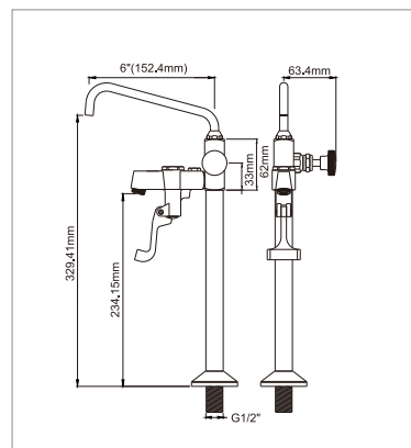
9850-AF Pedestal push back single glass filler
