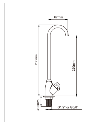
9854 Drinking Water Faucet
