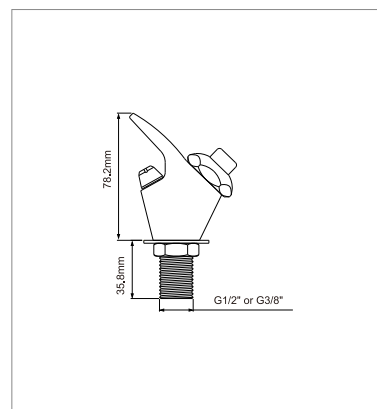
9853 Drinking Water Faucet
