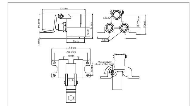
F-903A CAST KNEE VALVE
