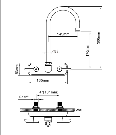
M98E-509SG03 4" (102mm) Center Wall Mounted Faucet with 5 11 / 16 " swivel gooseneck
