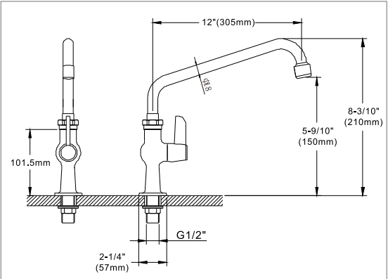
M98E-505SN12 Single supply deck mounted faucet
