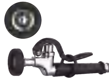
M0098SV-065G spray valve 0.65gpm@60psi
