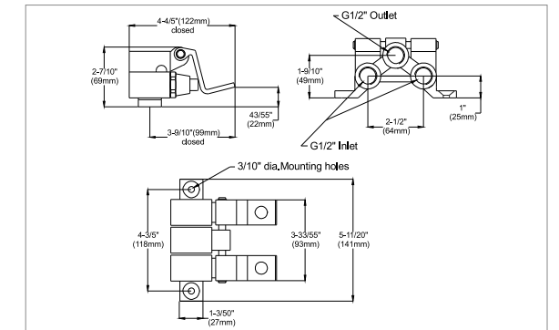
F-903 CAST DOUBLE FOOT VALVE
