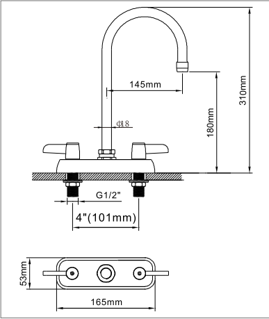
M98E-508SG03 4" (102mm) Center Wall Mounted Faucet with 5 11 / 16 " swivel gooseneck
