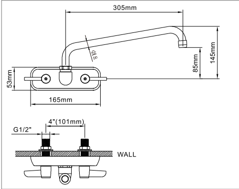
M98E-509SN12 4" (102mm) Center Wall Mounted Faucet
