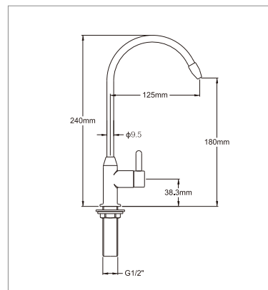
9855 Drinking water faucet
