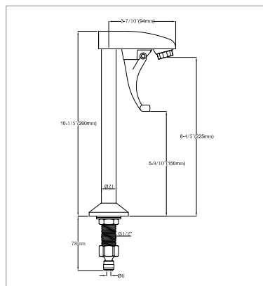
9850N Pedestal push back single glass filler
