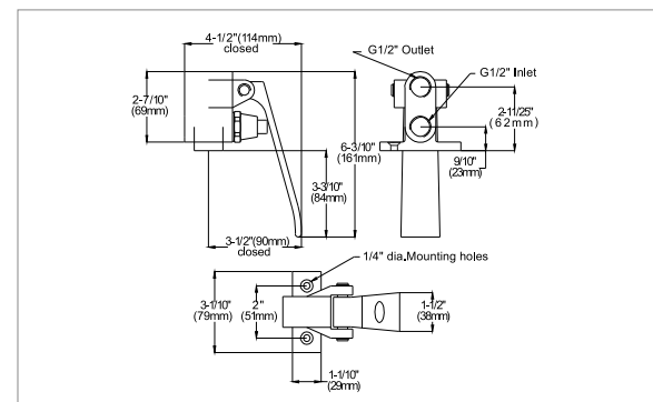
F-901 CAST SINGLE FOOT VALVE
