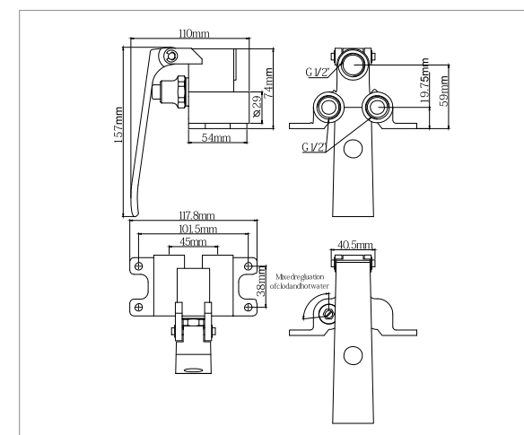
F-904 AUTO MIXING FORMED FOOT VALVE
