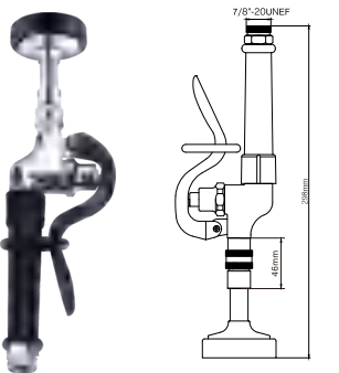
M-H098QC-SV Spray Valve Quick-Connect
