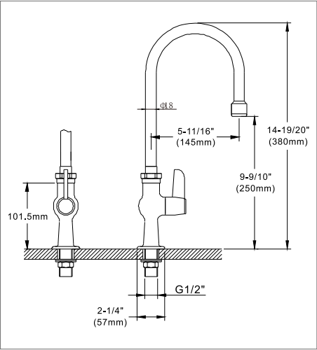
M98E-505SG03 Single supply deck mounted faucet with 5 11 / 16 " swivel gooseneck
