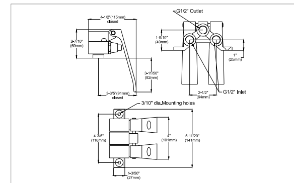
F-903 CAST DOUBLE FOOT VALVE
