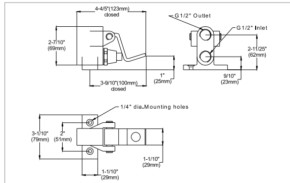
F-901 CAST SINGLE FOOT VALVE
