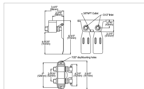
F-902 FORMED FOOT VALVE
