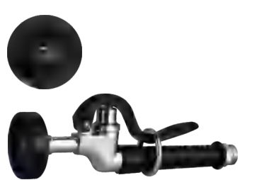
M0098SV-124G spray valve 1.24gpm@60psi
