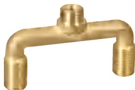
0098-H03 1)4"(102mm)Centers 2)1/2"NPSM male inlets 3)The product includes check valve to prevent cross-flow
